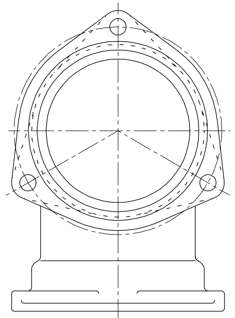
●寸法表(K-LL)
