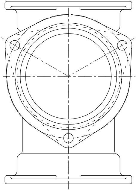
●寸法表(K-ST)
